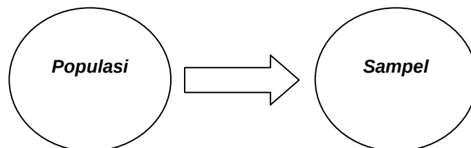
Gambar 9 : Random Sampling
