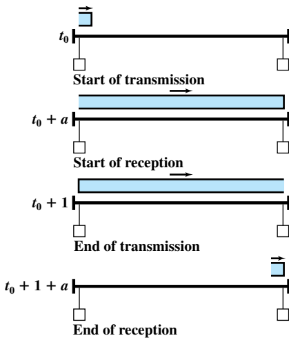
(a) Transmission time = 1; propagation time = a < 1 (b) Transmission time = 1; propagation time = a > 1
