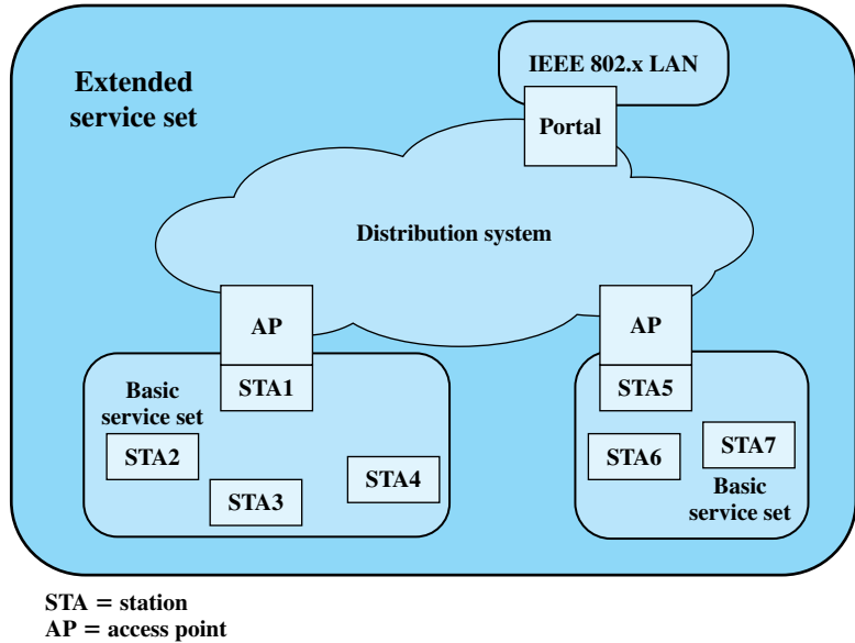
Figure 17.4 IEEE 802.11 Architecture
