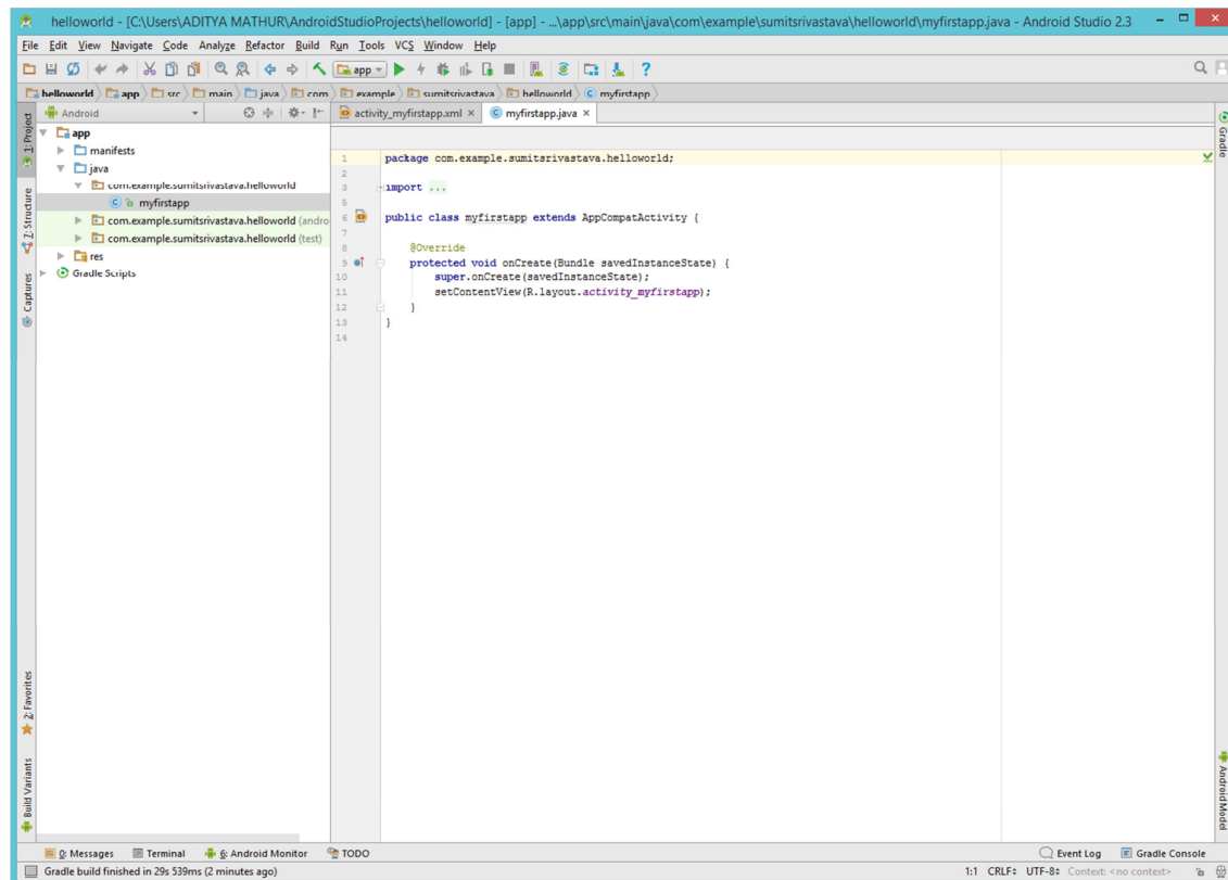
Figure 5.9: helloworld application
