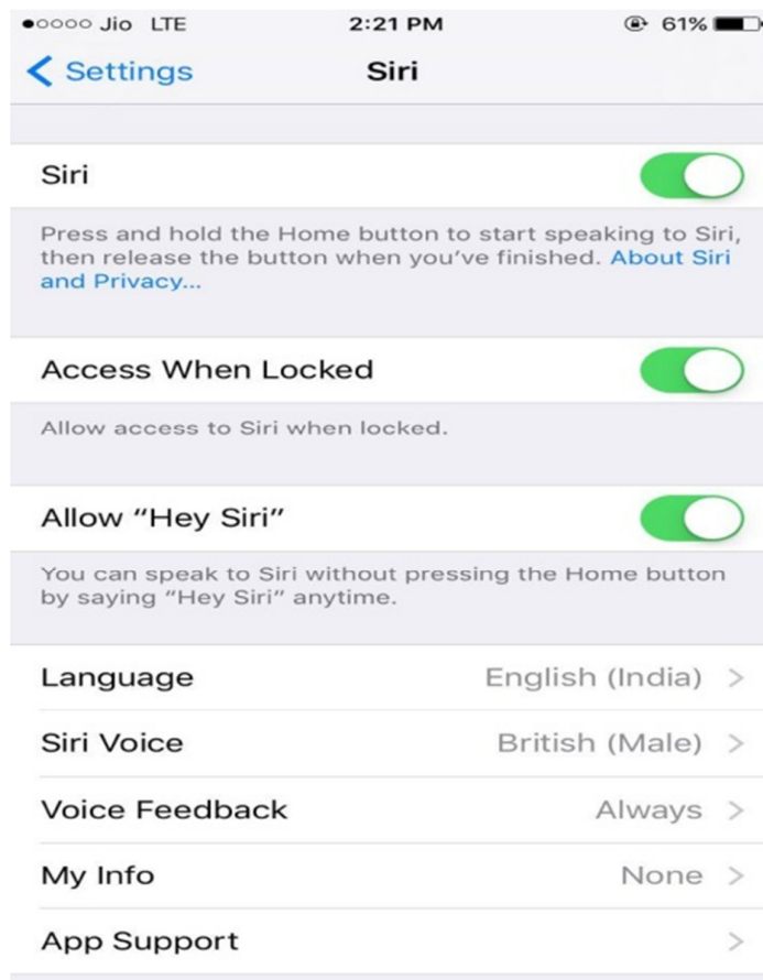
Figure 6.4 : Enabling Siri
