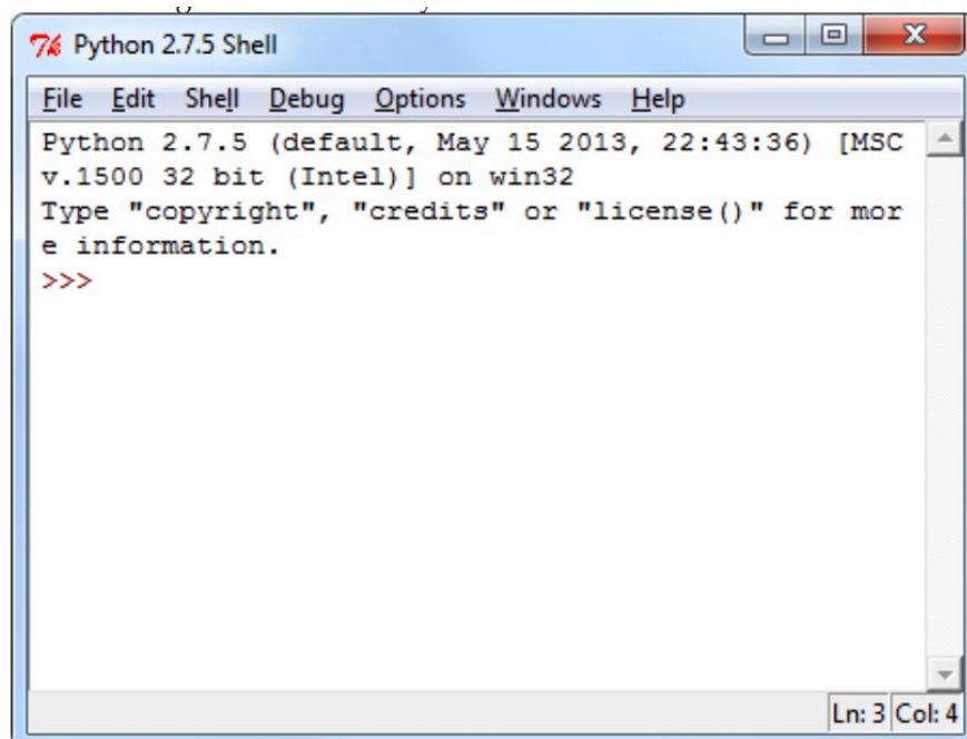
Fig. 3.2 Worksheet Python
