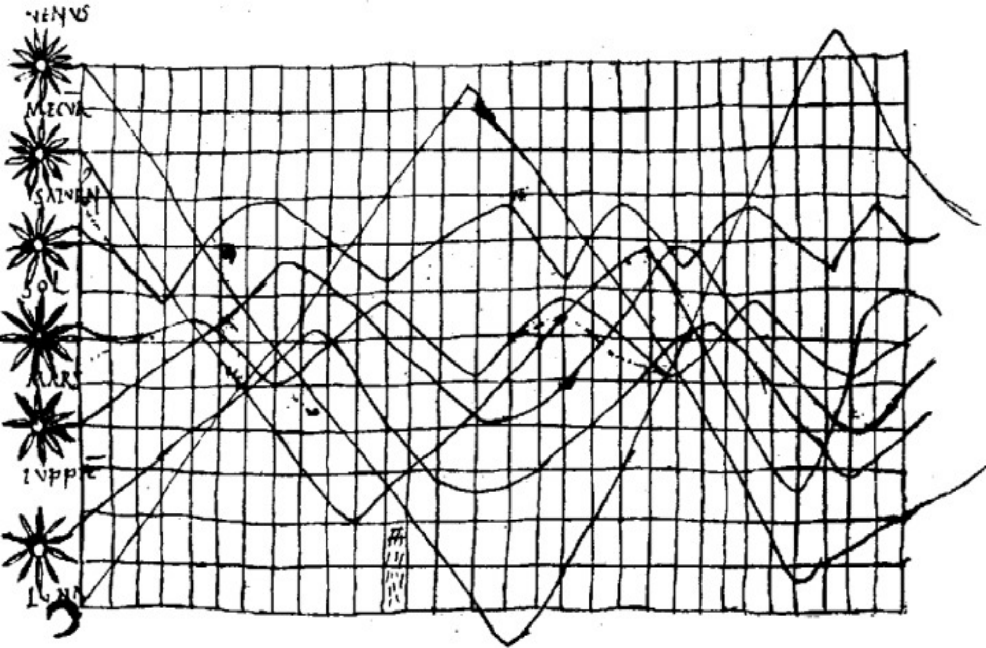
~950 AD Position of Sun, Moon and Planets
