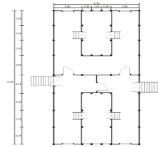
Gambar 1. Denah Rumoh T. Tjhik Mat Said
